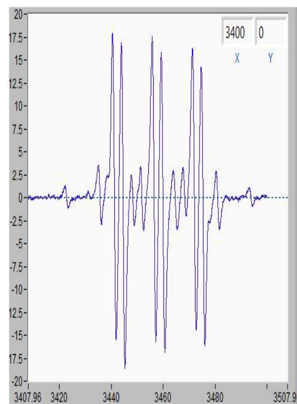
PBN-DMSO-OH spin adduct
