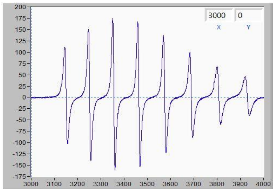
\text{VO}(\text{acac})_2 in \text{CHCl}_3
