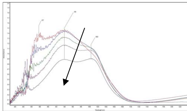
Figure 2. FT-NIR spectrum of C_{60}^{++} in oleum. The spectral evolution till 5 h after mixing show now a steady decrease in intensity as indicated by the arrow pointing downward. However, after 5 h the two bands at 938 nm and 1003 nm result stable for very long time.
