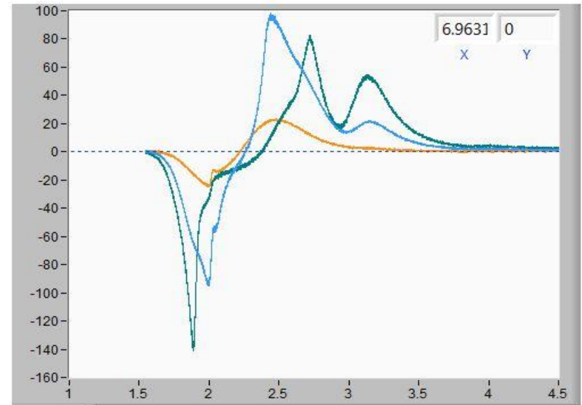
1, 5, and 10% solutions of ferrofluid in toluene
