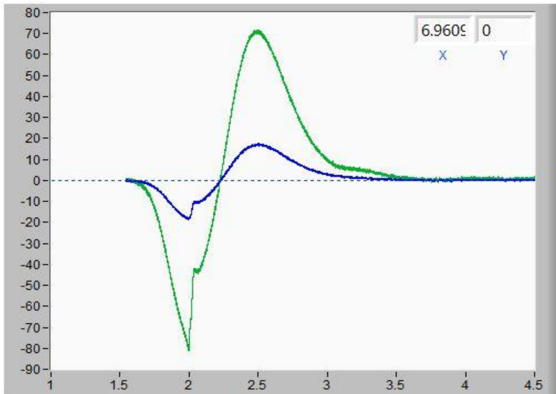
0.1 and 0.5% solutions of ferrofluid in toluene
